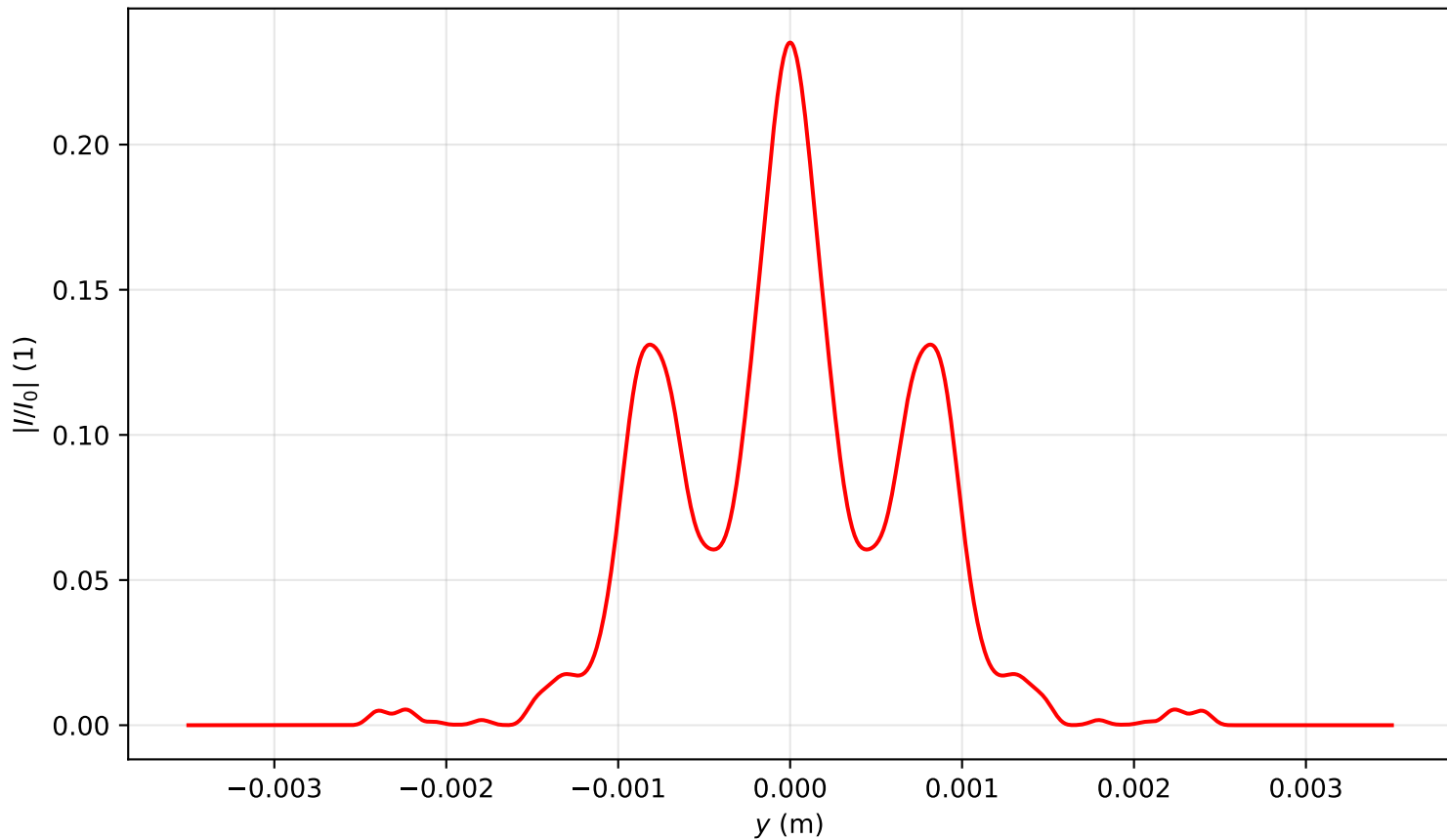
Intensity profile I(x=0, y, z=2.149)/I_0 , \text{Pin}=6.5\text{Pcr} , artificial time
